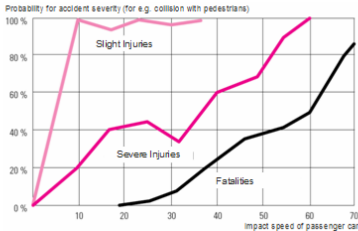
Figure 44: Accident Impact Speed and Severity of Injuries
